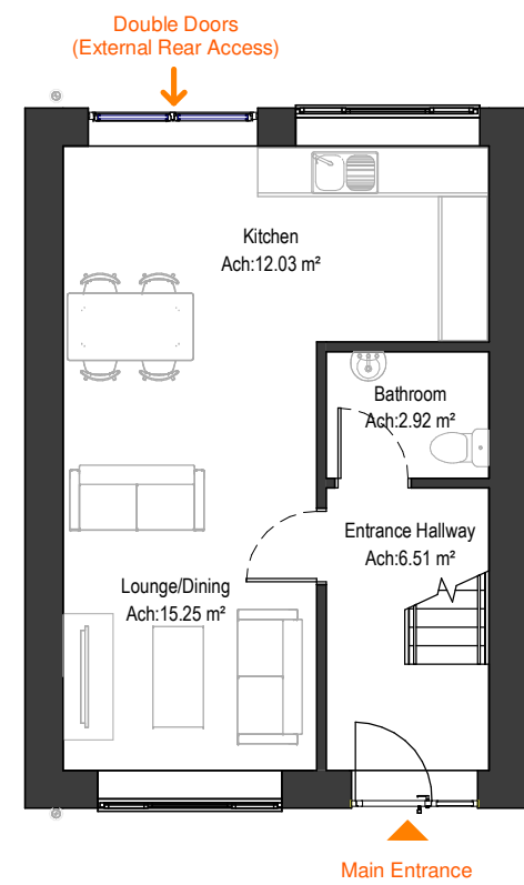
GF_H2 Ground Floor Plan 1 : 100
