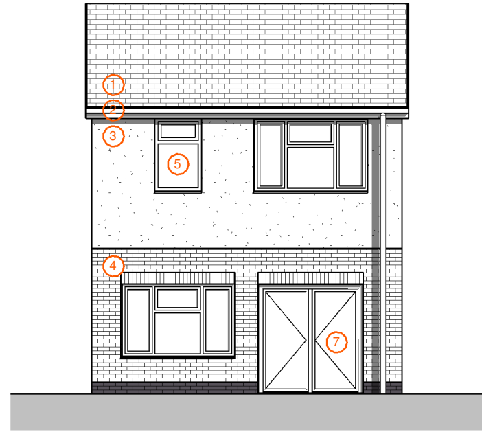
H2 Rear Elevation 02 1 : 100
