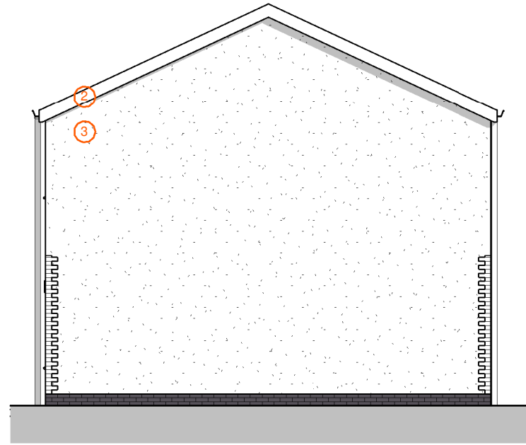
H2 Side Elevation 03 1 : 100
