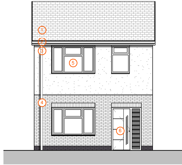
H2 Front Elevation 01 1 : 100
