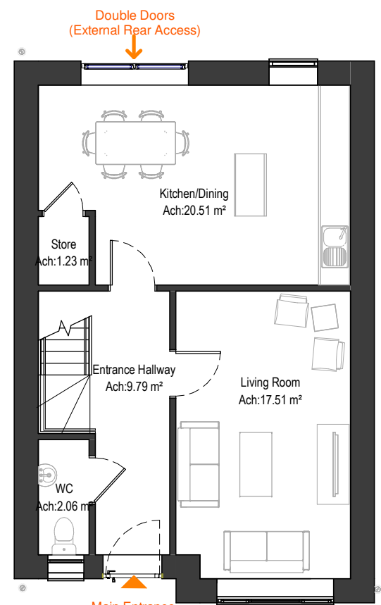
GF_SSA H3 A Ground Floor Plan 1 : 100
