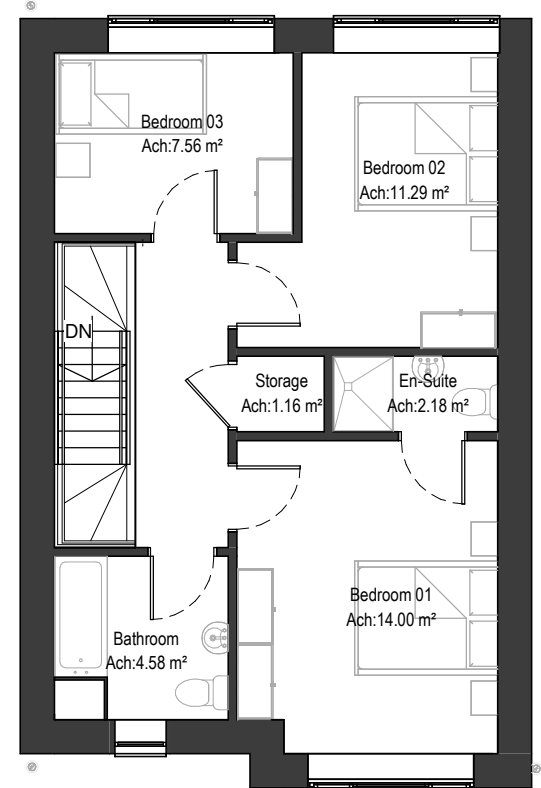
FF_SSA H3 A First Floor Plan 1 : 100
