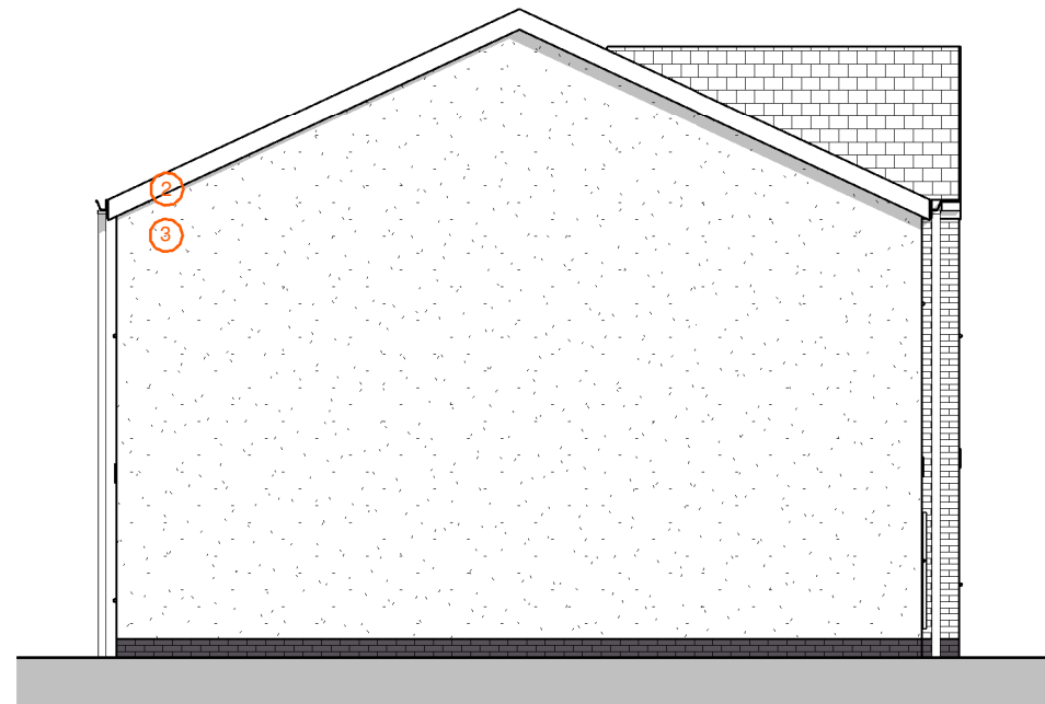
SSA H3 A Side Elevation 03 1 : 100
