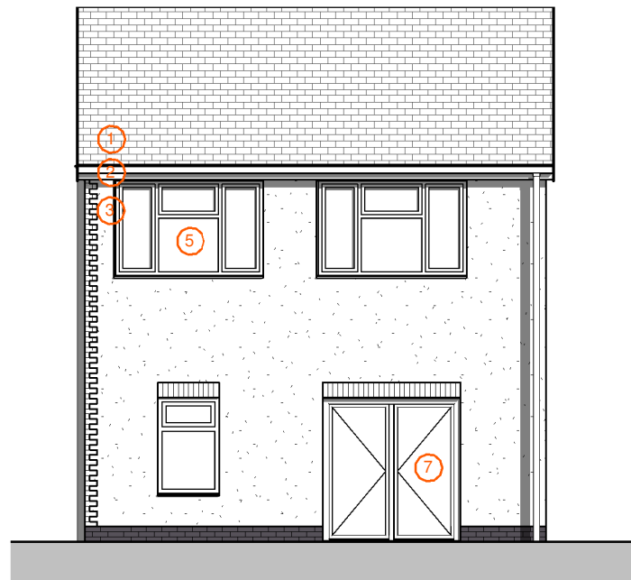
SSA H3 A Rear Elevation 02 1 : 100
