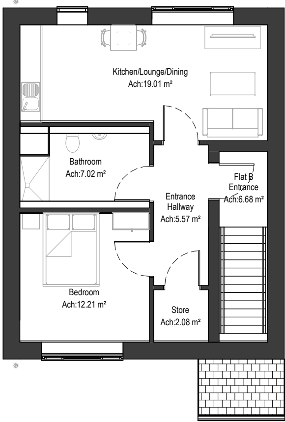
FF_F2.2 First Floor Plan 1 : 100
