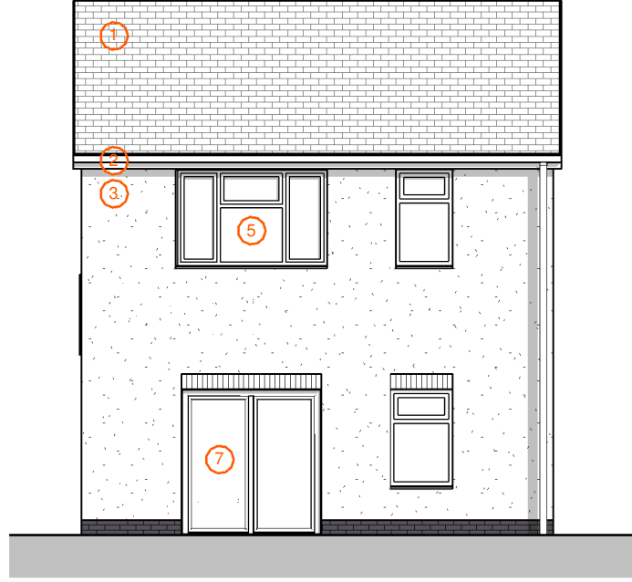
F2.2 Rear Elevation 02 1 : 100
