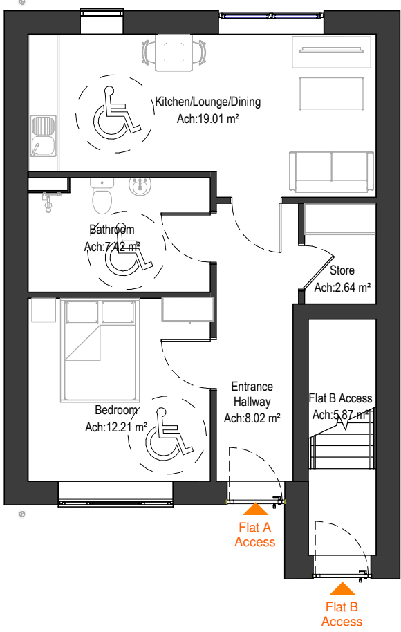
GF_F2.2 Ground Floor Plan 1 : 100
