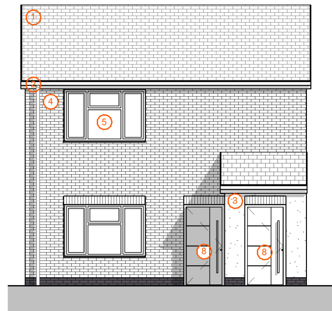
F2.1 Front Elevation 01 1 : 100
