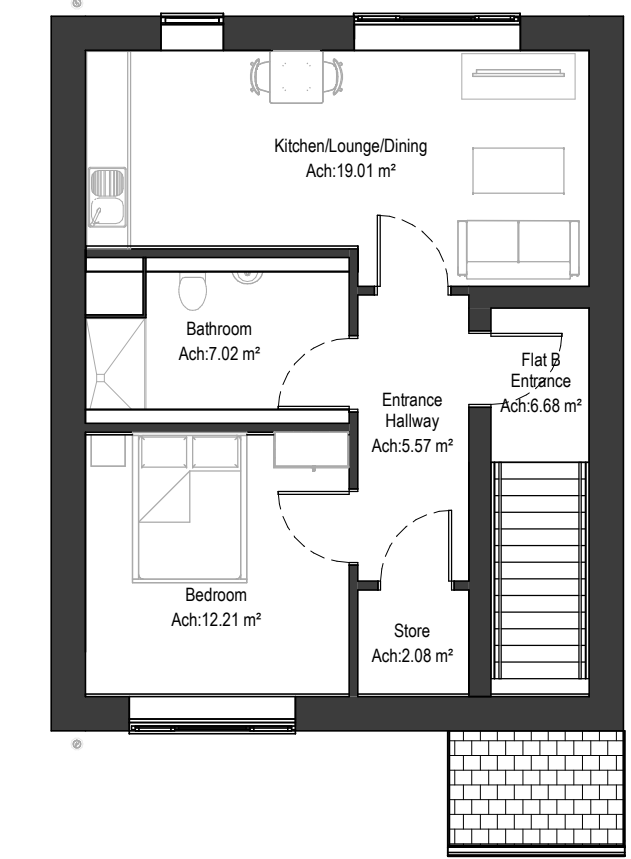
FF_F2.1 First Floor Plan 1 : 100
