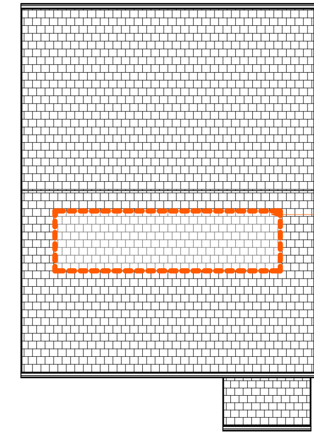
RF_F2.1 Roof Plan 1 : 100
