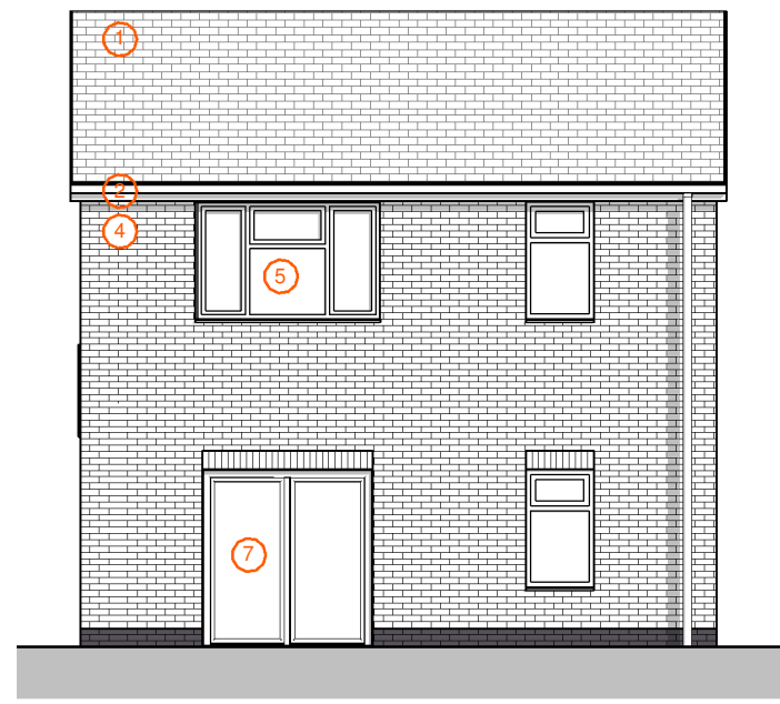
F2.1 Rear Elevation 02 1 : 100
