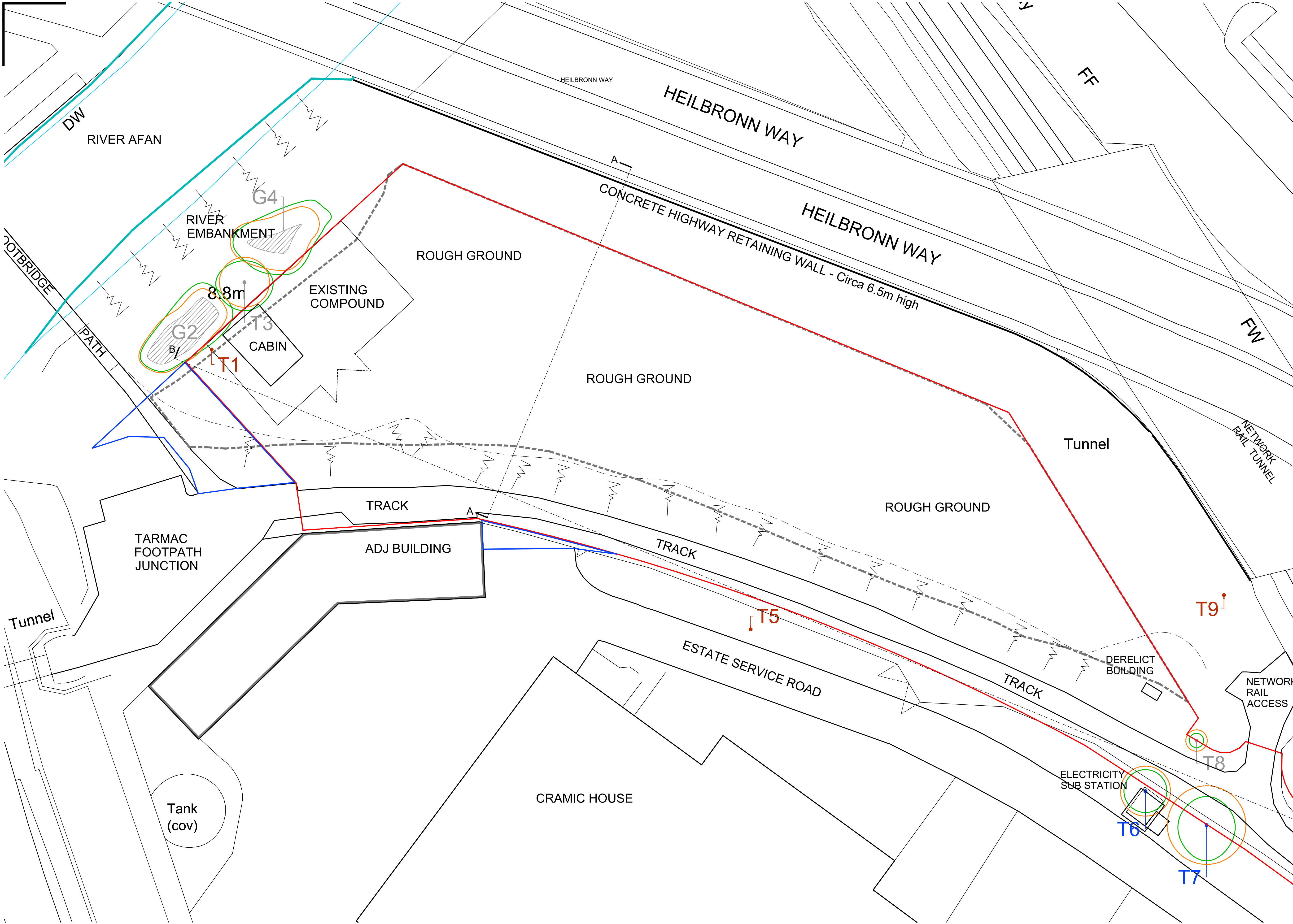
EXISTING SITE LAYOUT Scale 1:250
