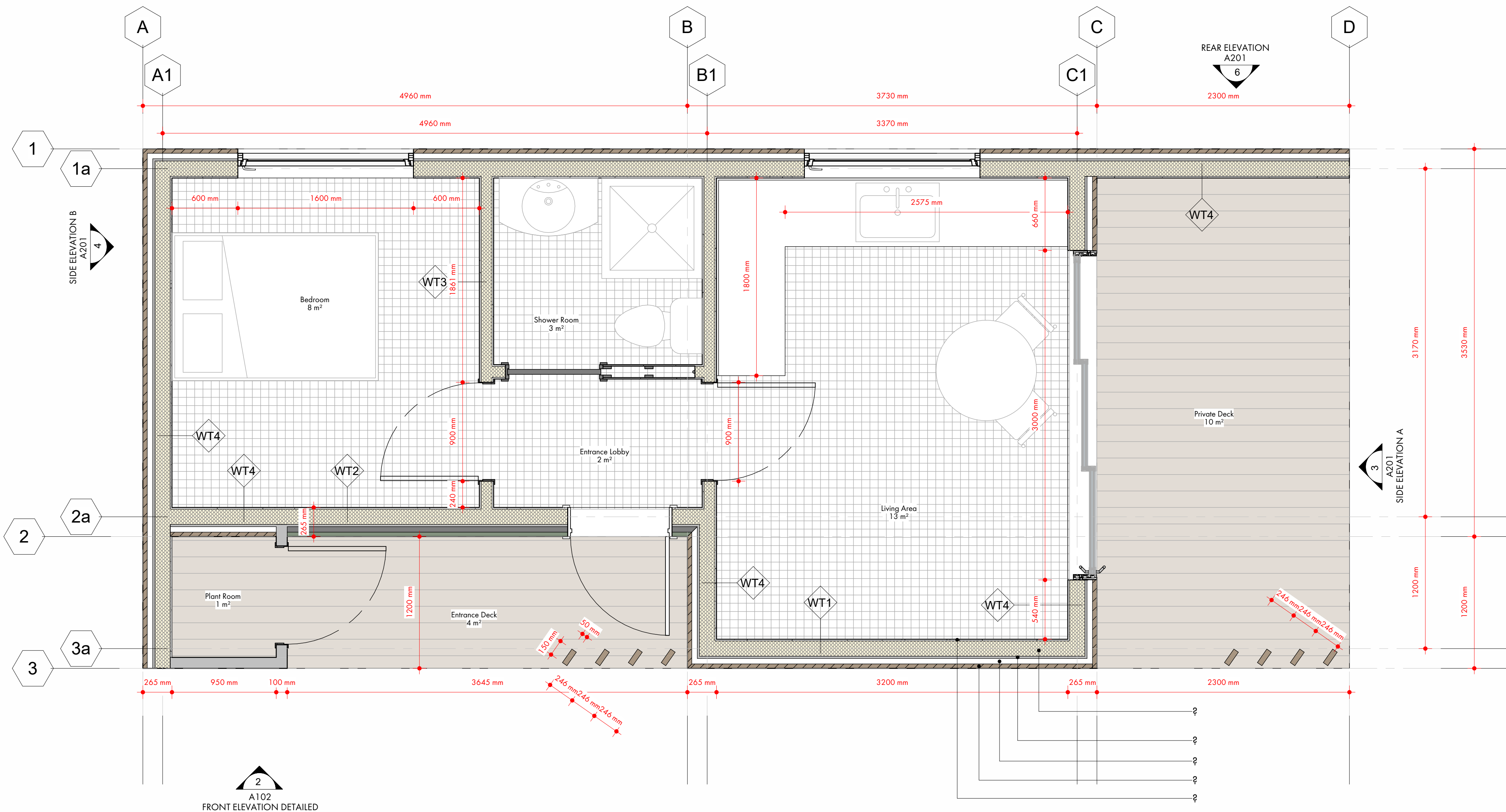
View No. 1 Sheet A102 DETAILED LAYOUT 1 : 25
