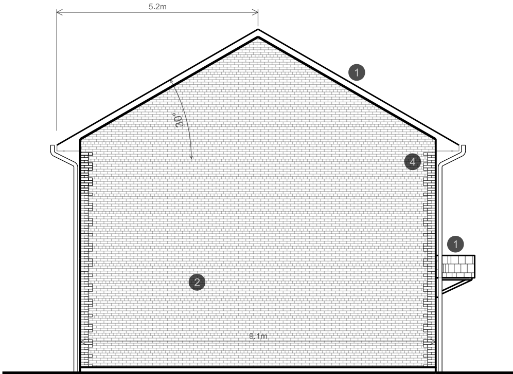
Type H3 - 5P2B Left Elevation
