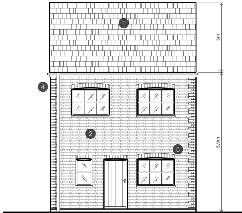
Type H3 - 5P2B Back Elevation
