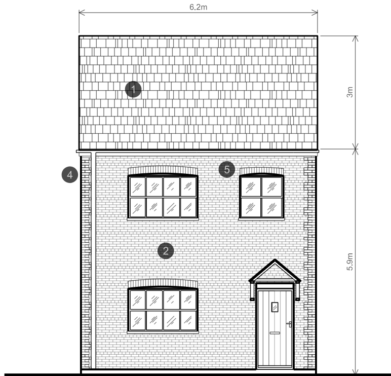
Type H3 - 5P2B Front Elevation
