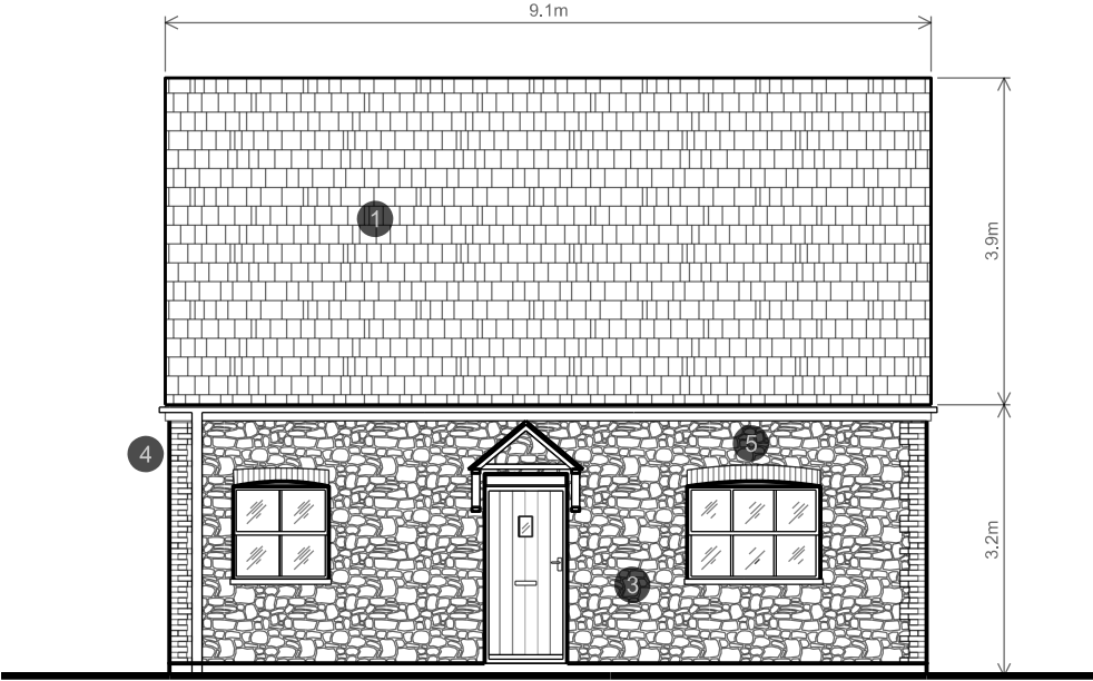
Type B1 - 3P2B - Bungalow Front Elevation
