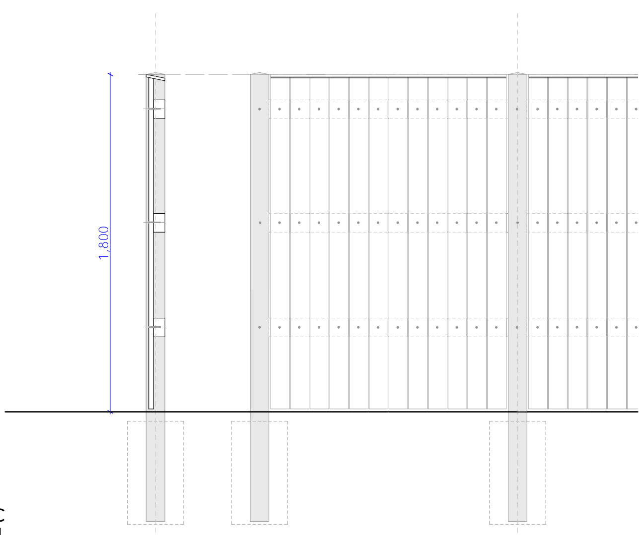
Fence Type C 1:20 @ A1
