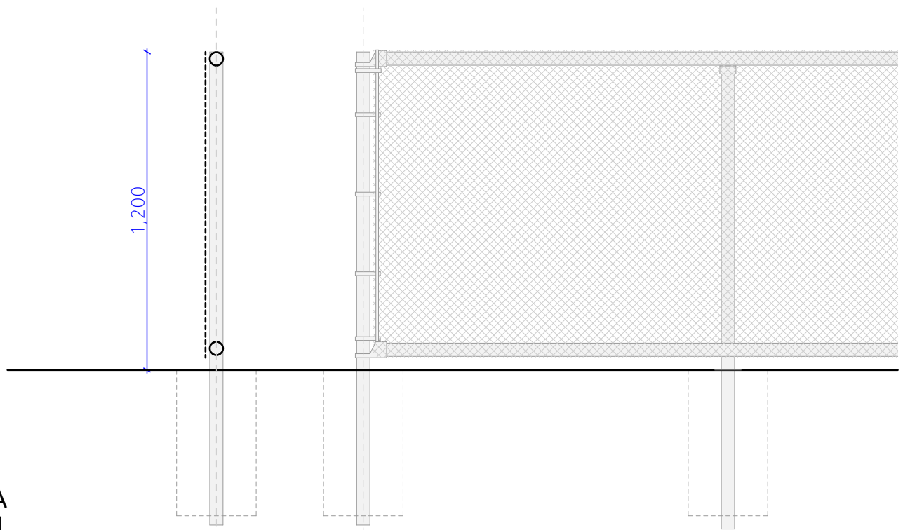
Fence Type A 1:20 @ A1
