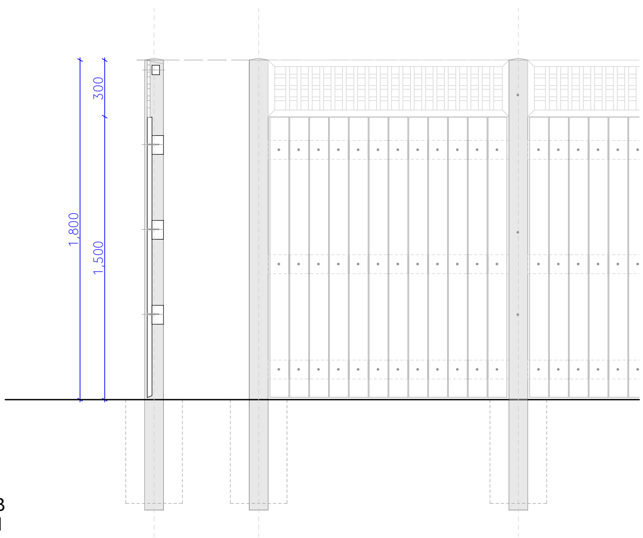
Fence Type B 1:20 @ A1
