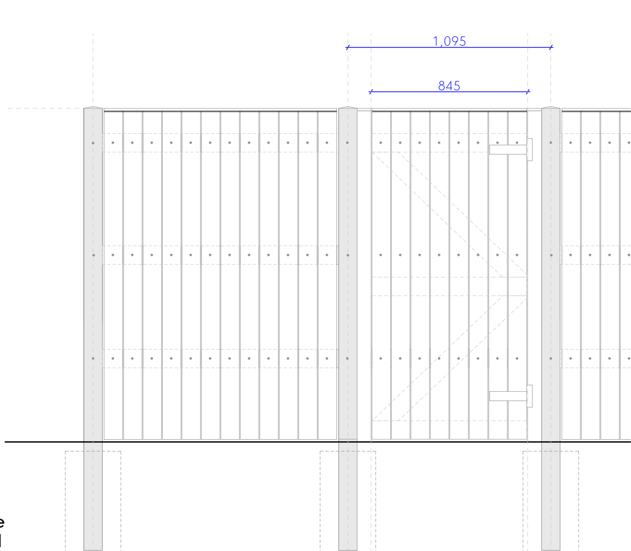
Fence Type C Gate 1:20 @ A1
