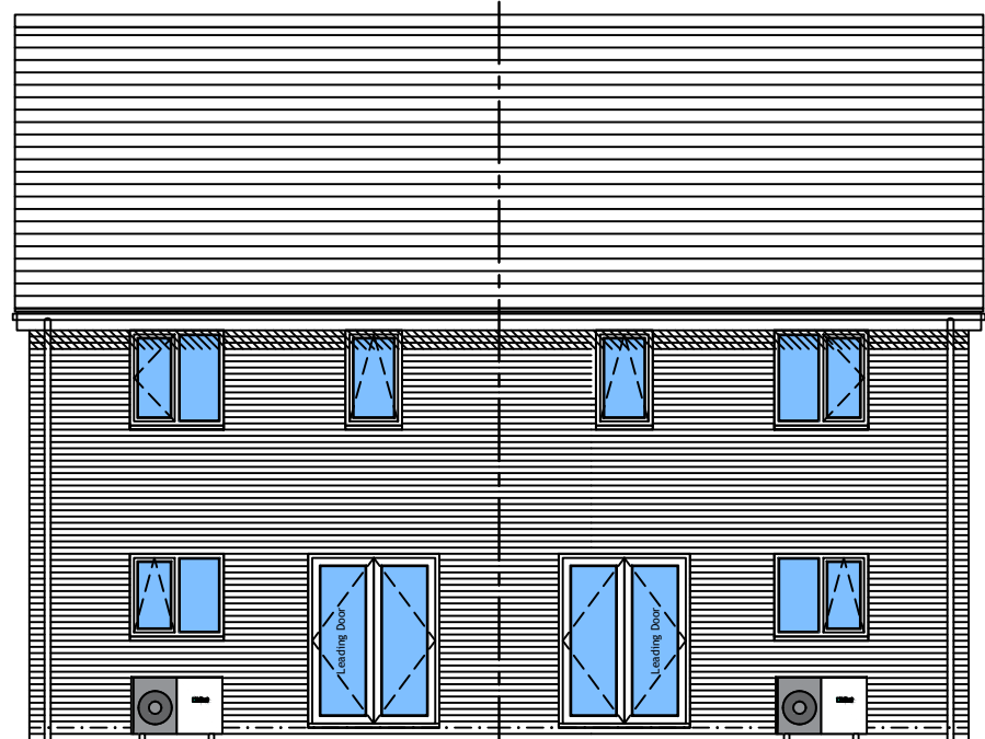
2.22 Rear Elevation / Drychiad Cefn
