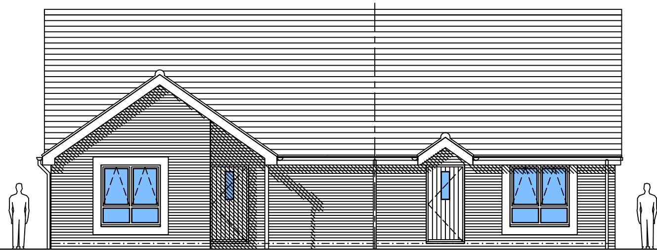
2.20 Front Elevation / Drychiad Blaen
