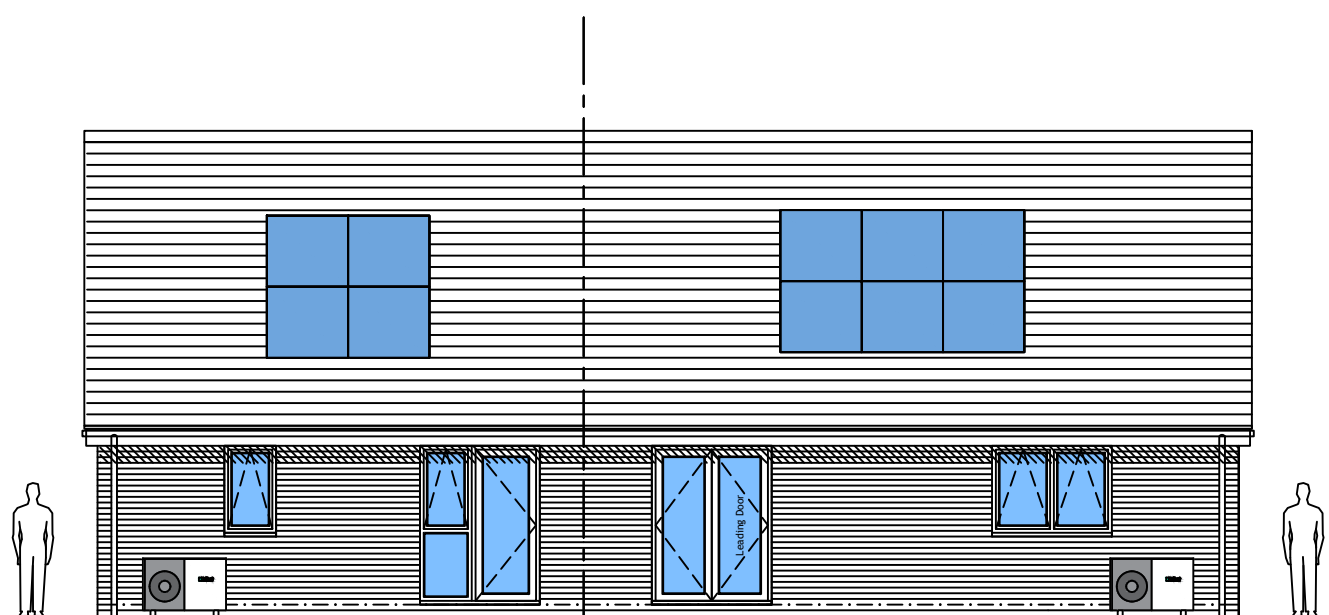
2.22 Rear Elevation / Drychiad Cefn
