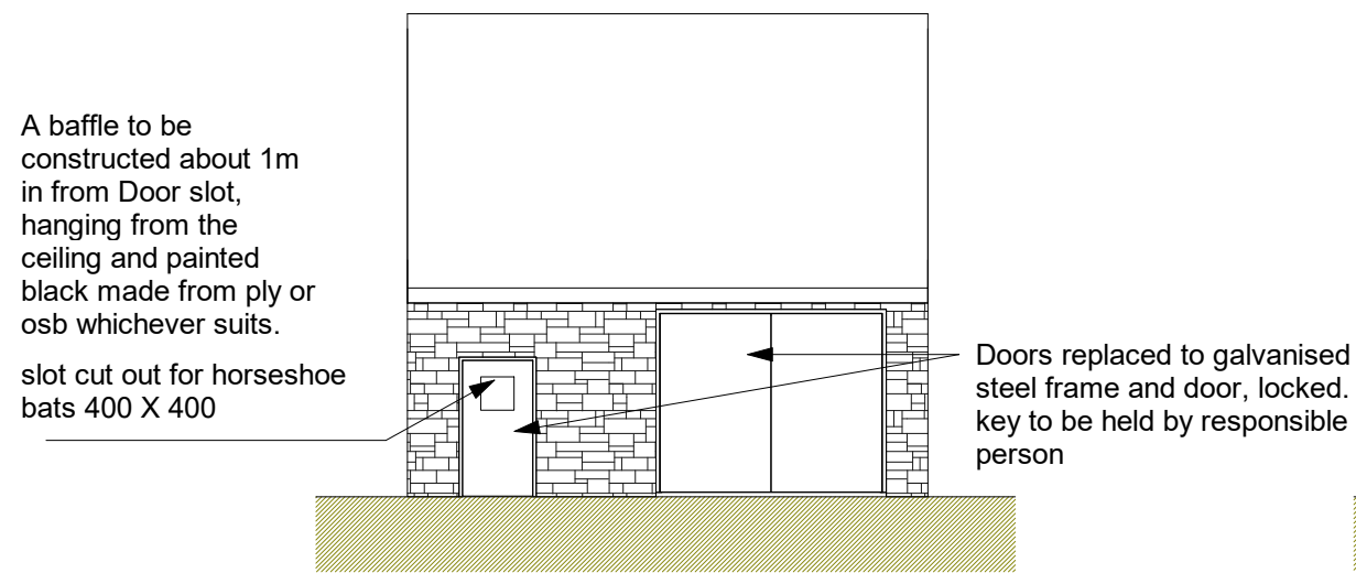
2 Front elevation 1 : 100
