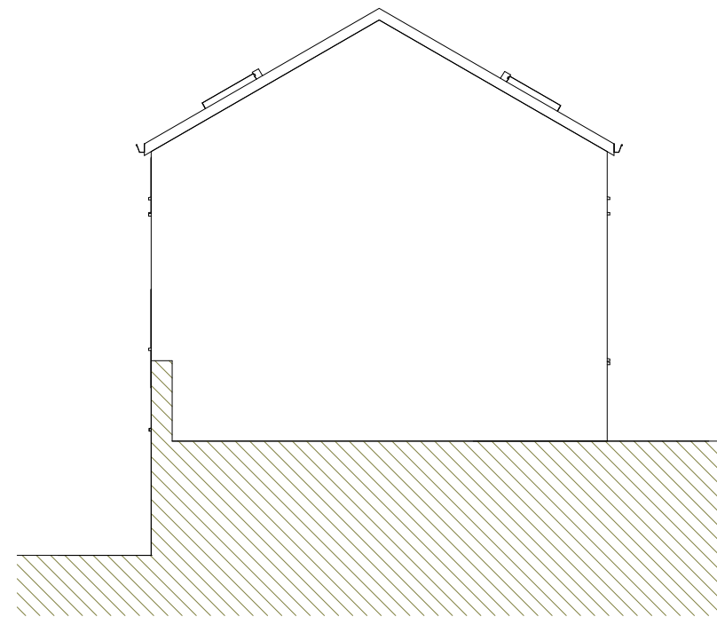
4 South East 1 : 100
