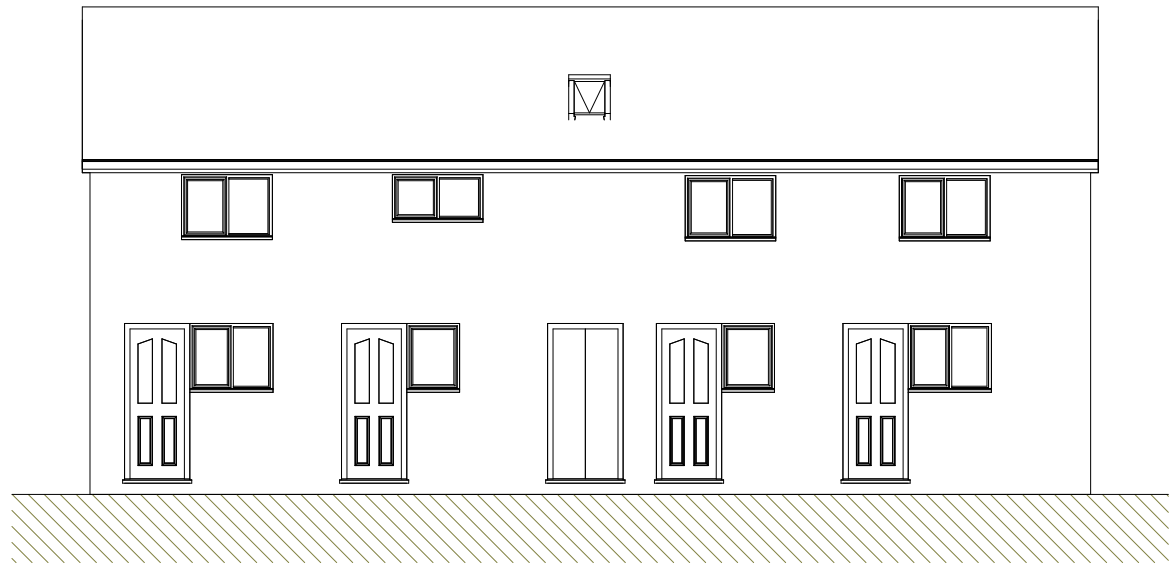
1 North East 1 : 100
