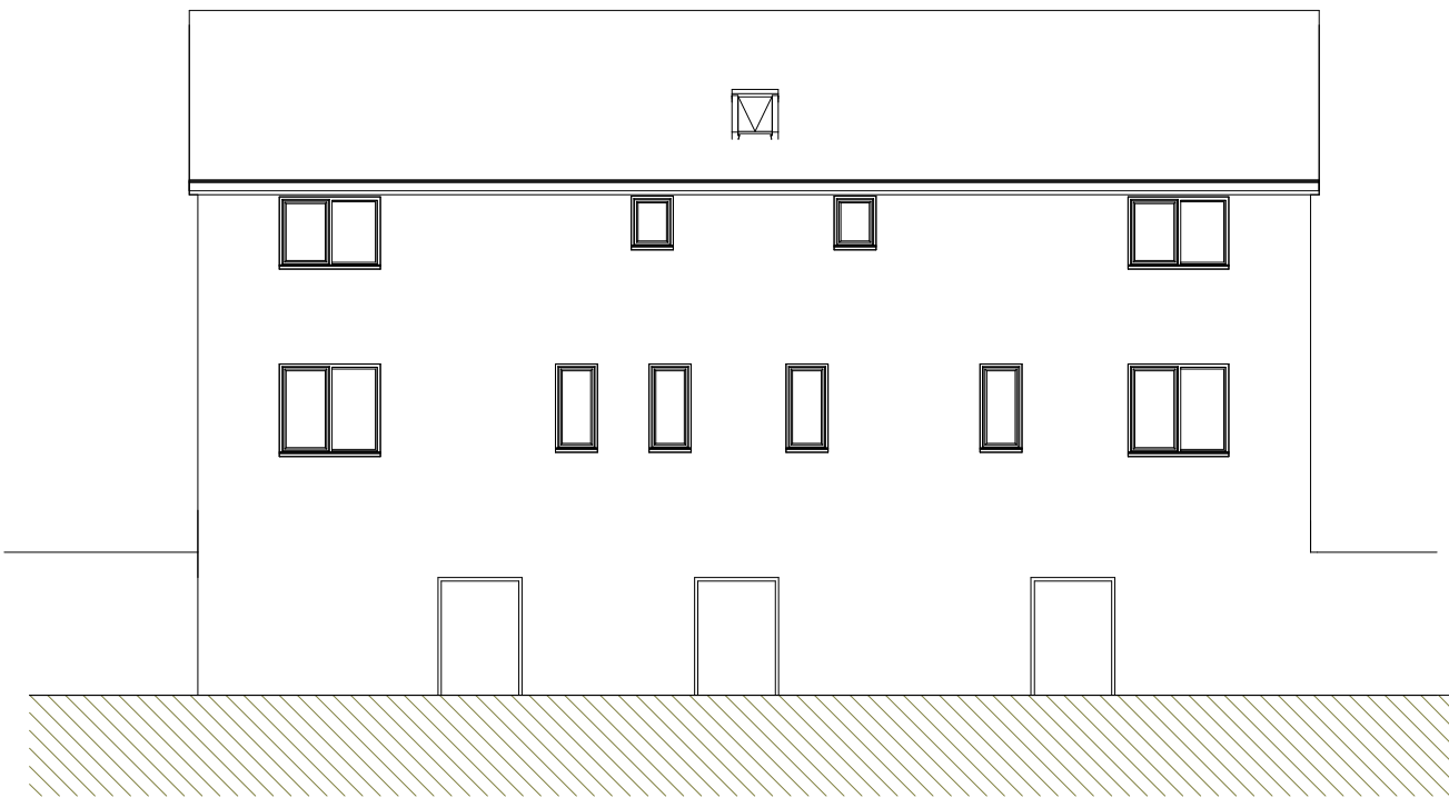
3 South West 1 : 100
