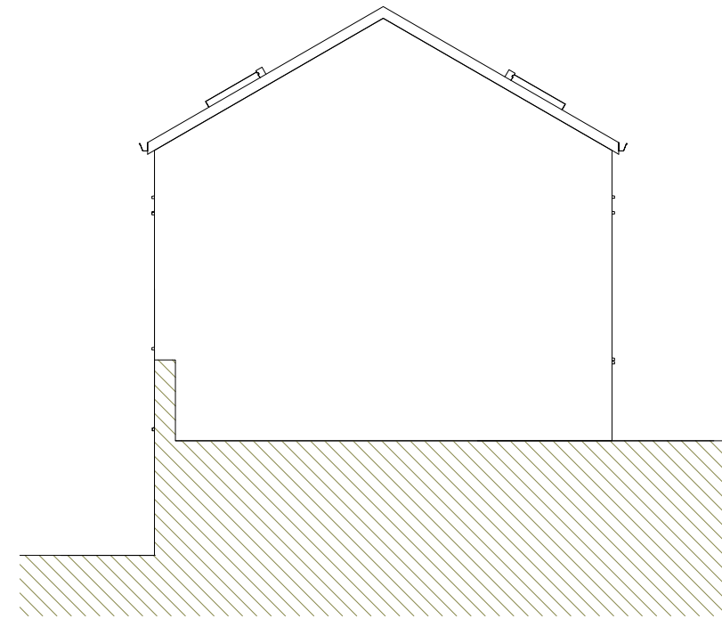
4 South East 1 : 100
