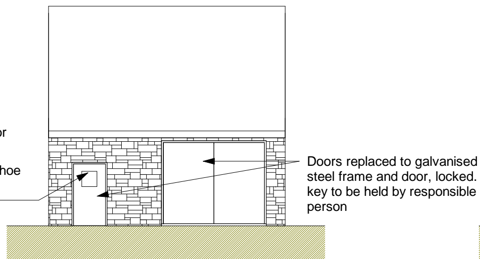
2 Front elevation 1 : 100
