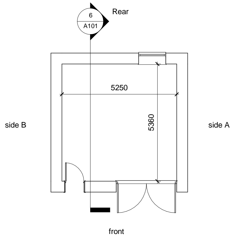
1 ground floor 1 : 100
