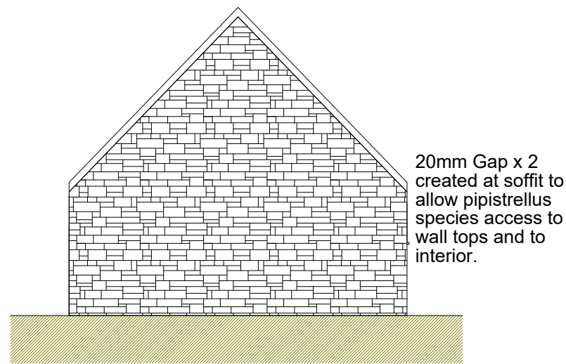
3 Elevation on A 1 : 100
