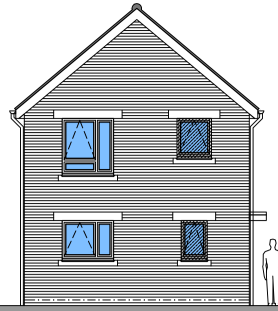
2.20 Front Elevation
