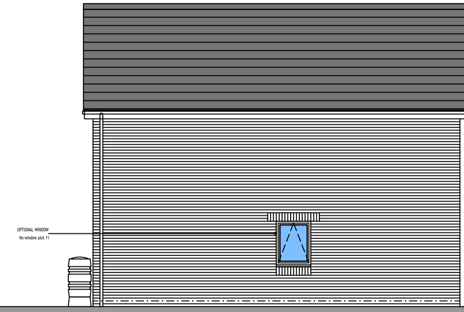
2.21 Left Hand Side Elevation
