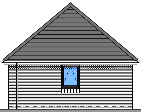
2.21 Left Hand Side Elevation
