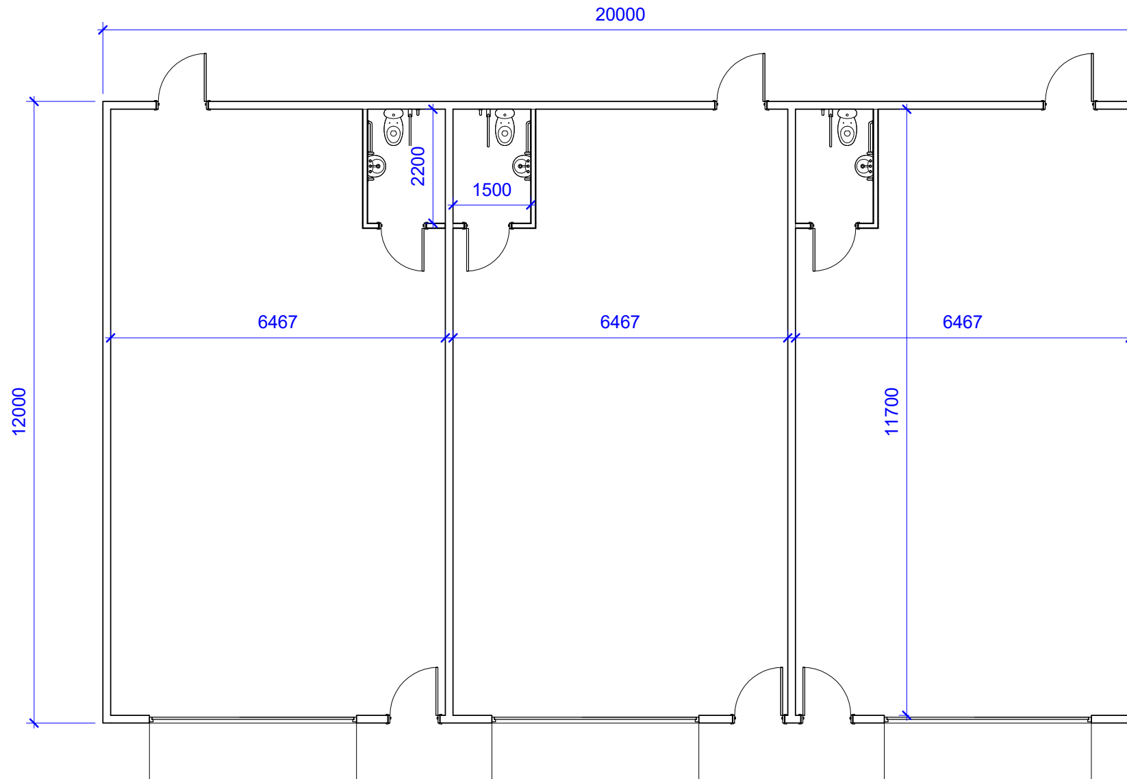
1 ground floor 1 : 100
