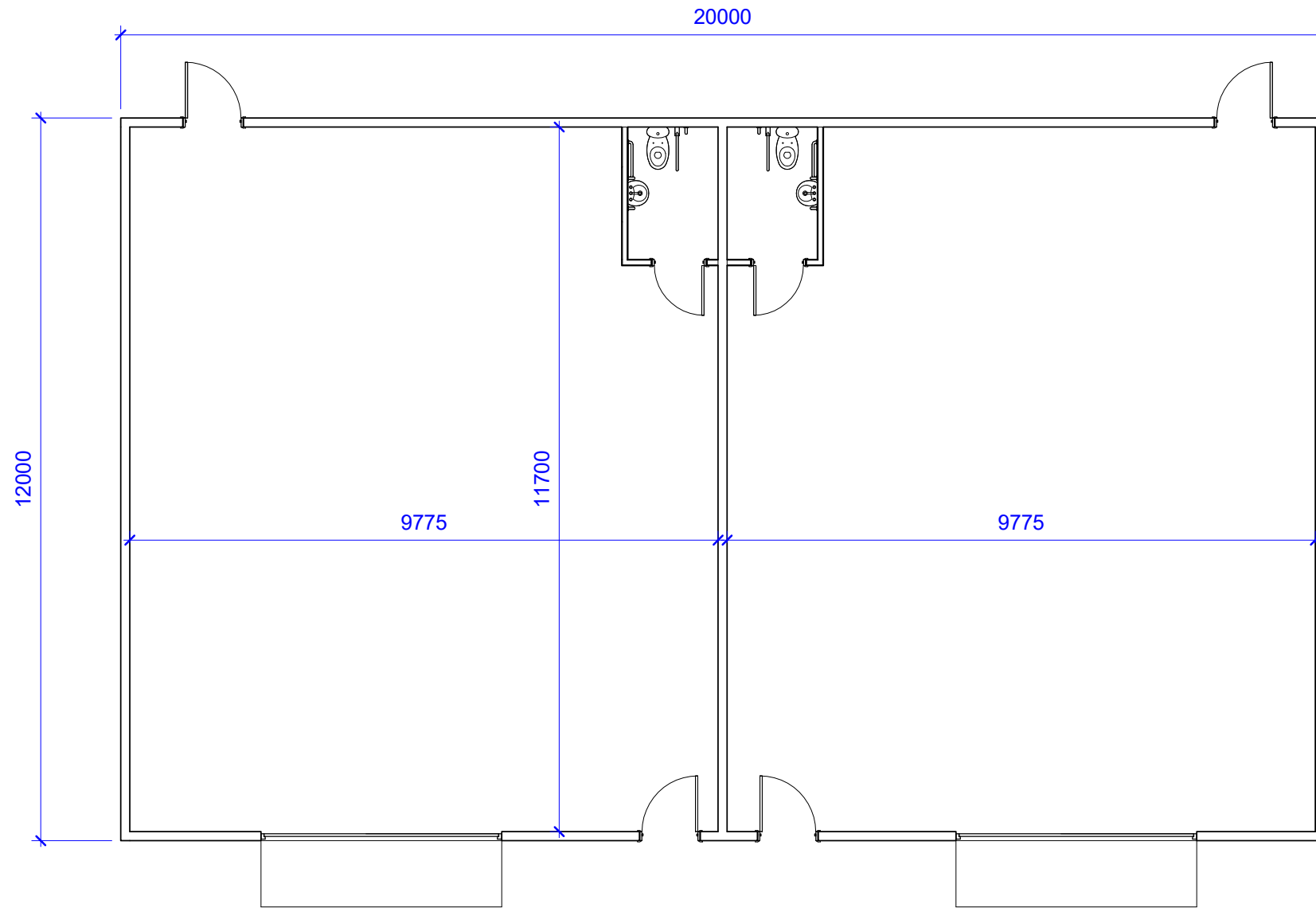
1 ground floor 1 : 100
